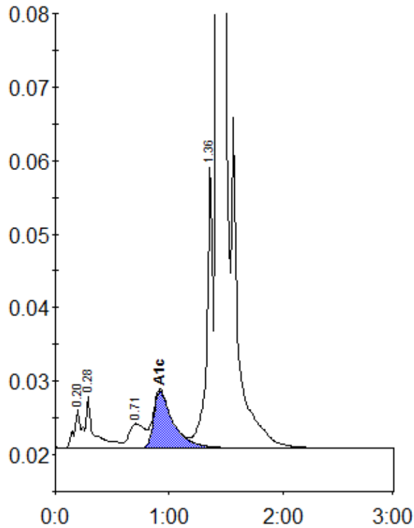
Peak table - ID: 10528313
